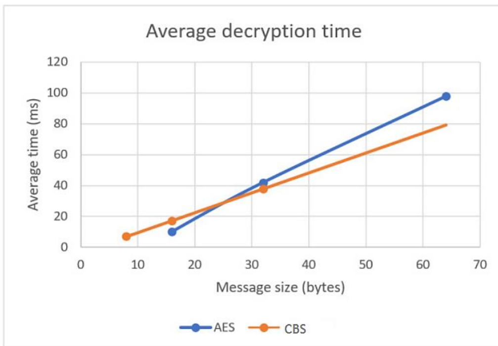
Fig 5 - Average Decryption Time
